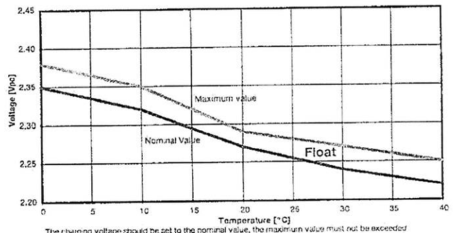
Fig. 1: Marathon L/XL and Powerfit S100/S100L/S300; charging voltage vs. temperature
